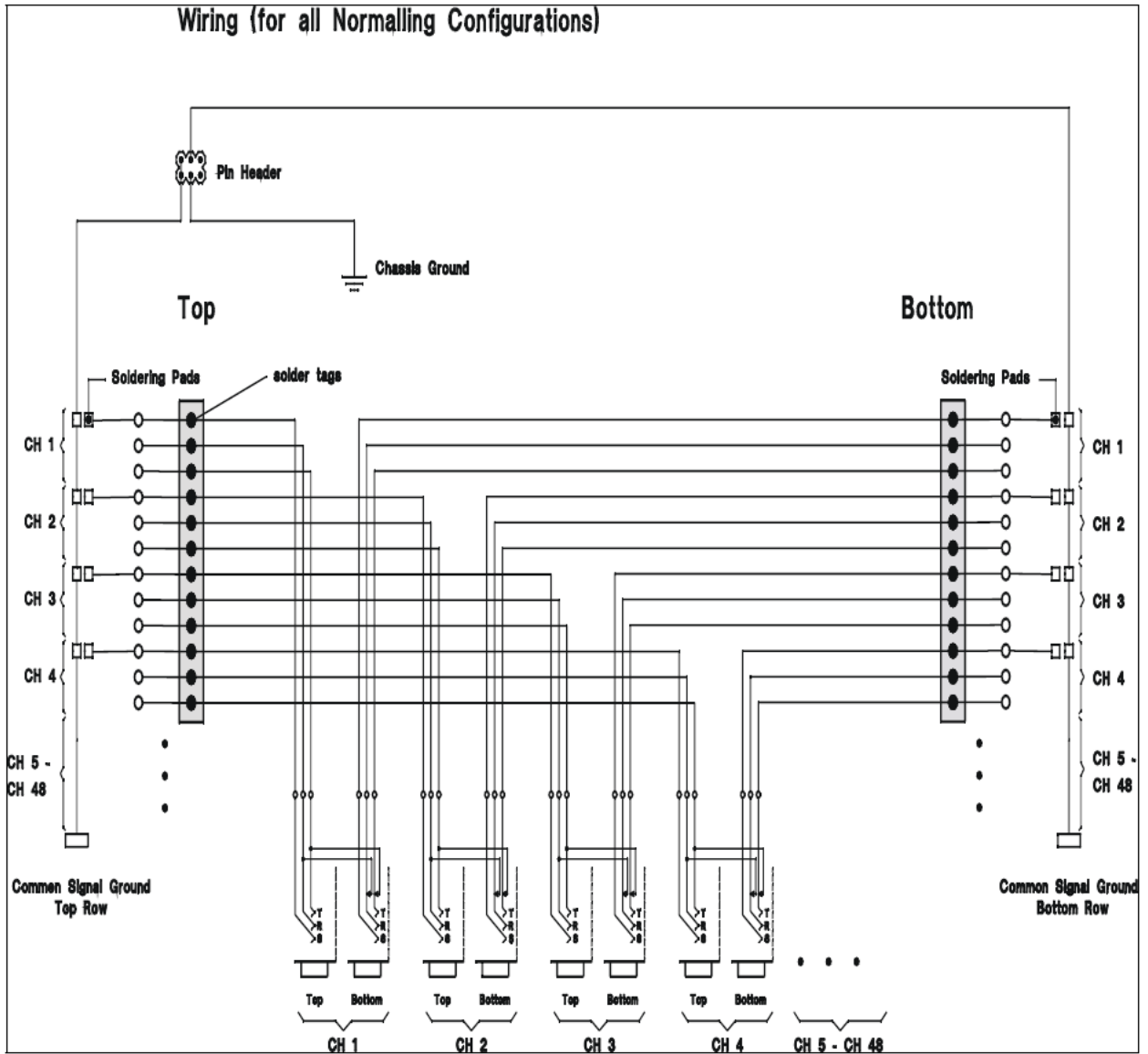
Wiring diagram
